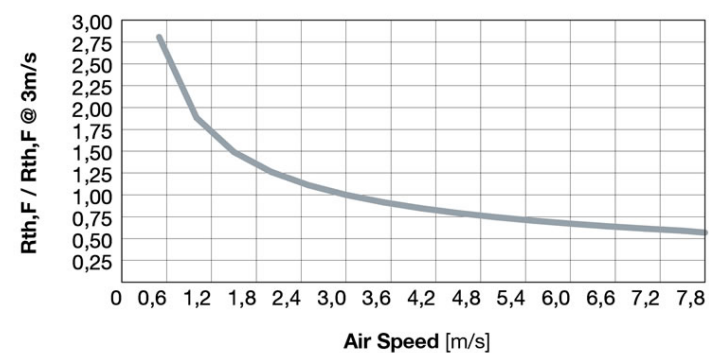
Air speed correction factor
