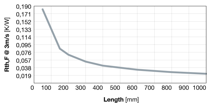
Thermal Resistance - Forced convection
